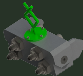
Outboard DWT Hot-Stab™ four port
